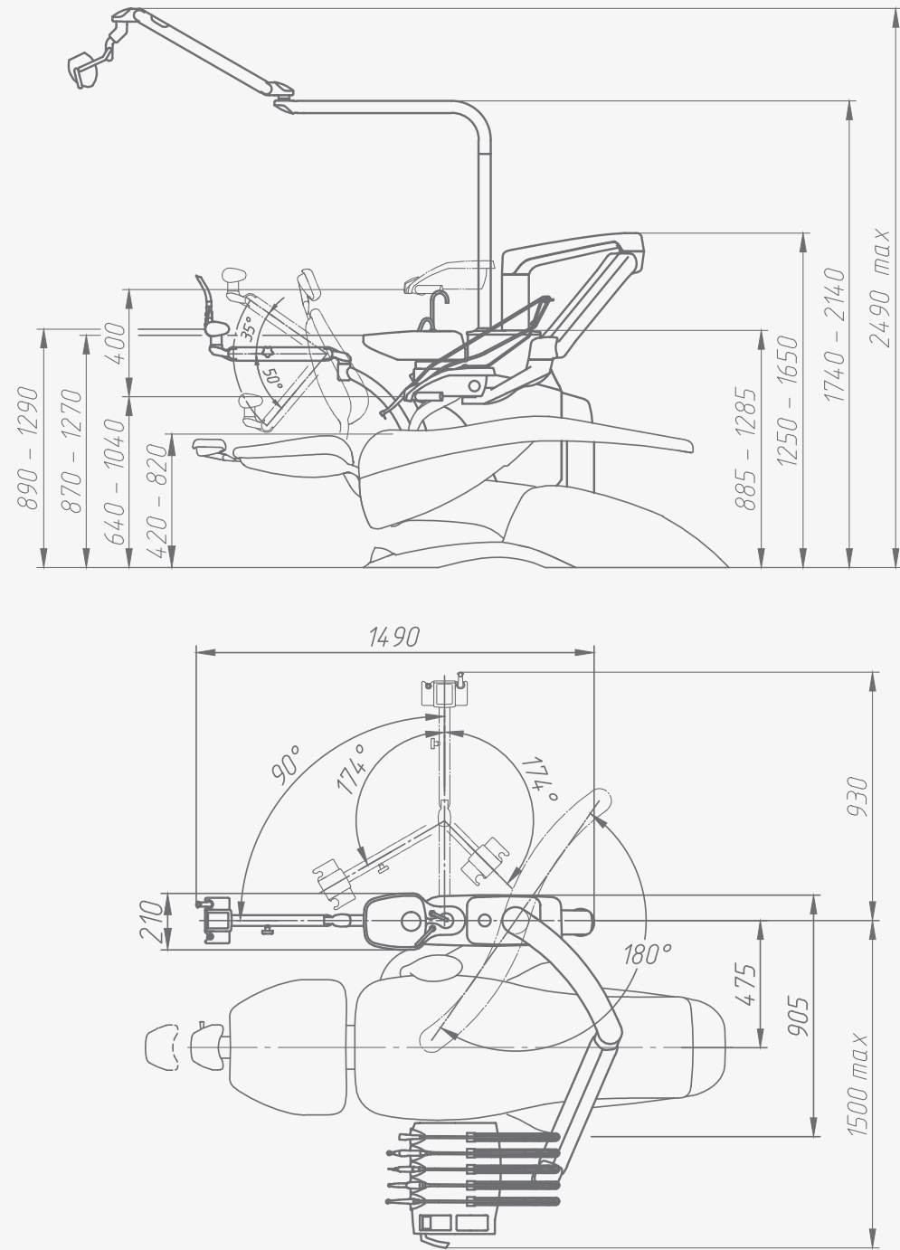
Overall dimensions of hanging dental unit GALLANT OMNIPRATIQUE with upper delivery of instruments and patient chair STING
